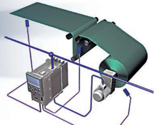
DEROULAGE ASYNCHRONE A TENSION CONSTANTE
