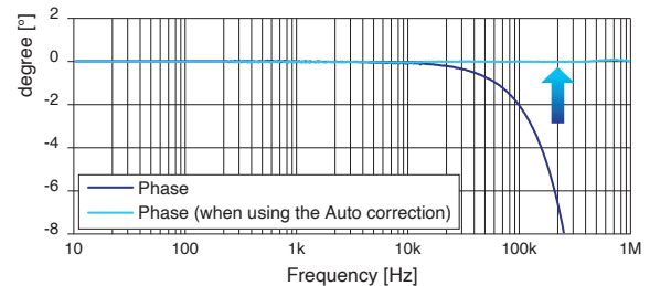
Example of the automatic phase correction for the CT6904A AC/DC current sensor
