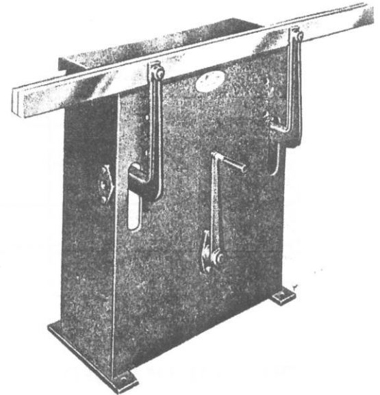
58-B-60 Filing clamp for 1.524 mm jaw band blades.
