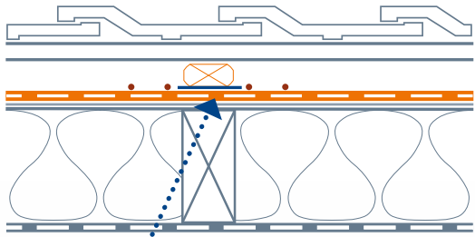
THERMO NAILTAPE (CLASSE 2)
