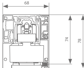
fixation murale 44 mm
