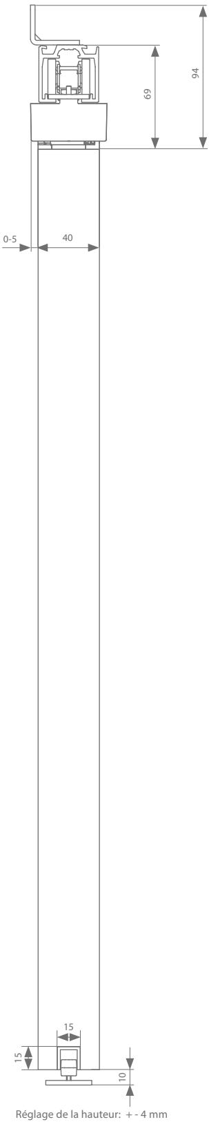
fixation murale 40 mm
