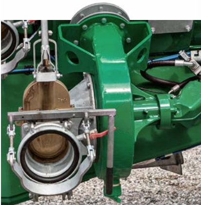
Side-mounted filling pump* Side-mounted filling pump with manual slide valve and quick hose coupling.
