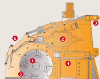
Marteaux fixes BSC
