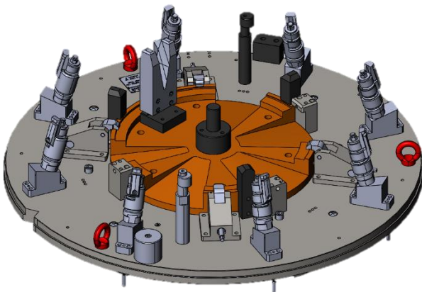
Etude outillage
