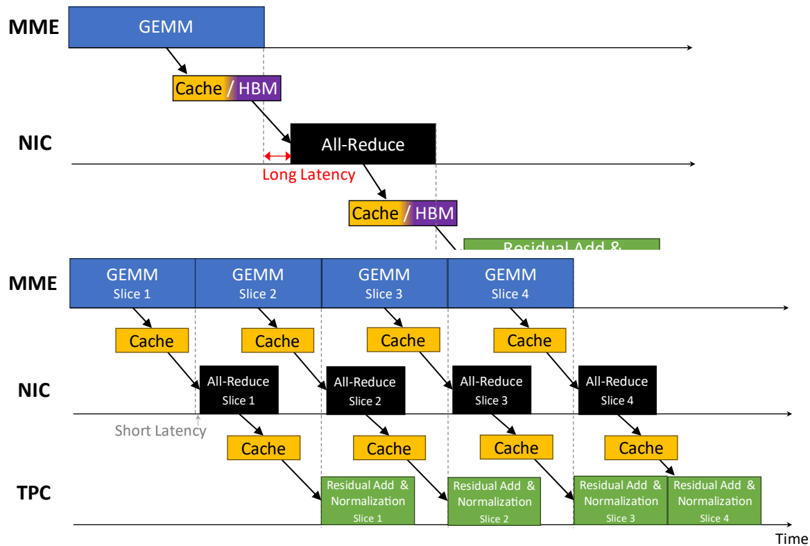
Figure 25. Optimized scheduling of the MME, NIC and TPC, with a producer-consumer relation between all three engines
