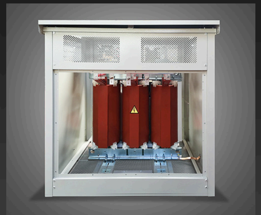
Cast resin 20 kV
