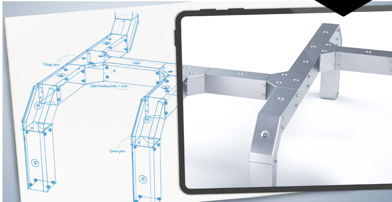
Design of component assemblies using easyRoute 3D system
