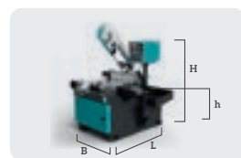
BS 350 SHI B 1480 mm L 1750 mm H 1900 mm h 940 mm Kg 649
