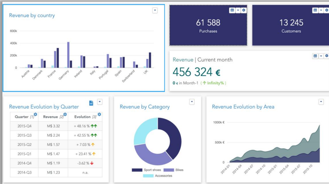
Dashboard view
