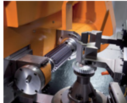
Automated gear cutting machine, production of spiral bevel gears
